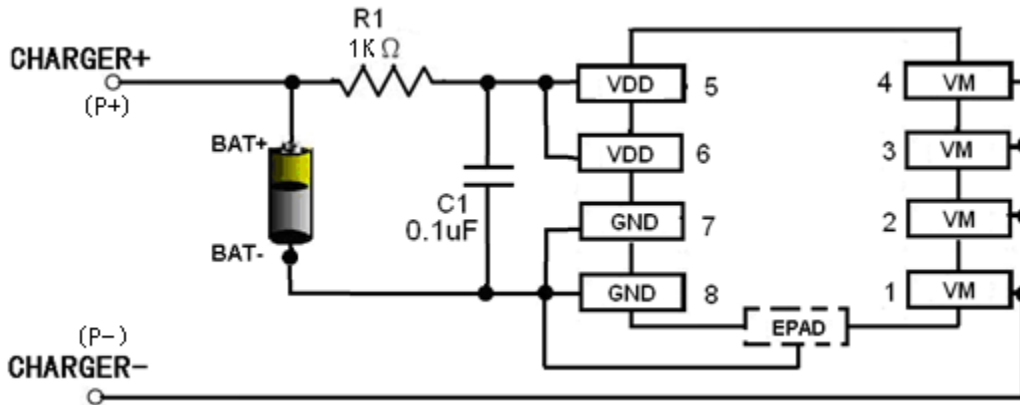
Fig 6 XB8887A in a Typical Battery Protection Circuit
